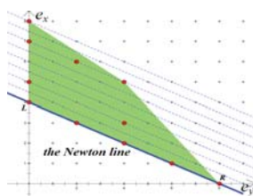
Figure 1: The polytope and the Newton line
