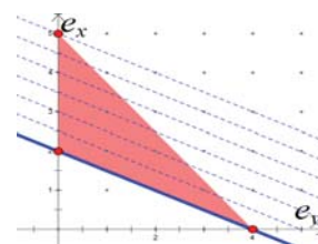
Figure 2: Lifting for G_2
